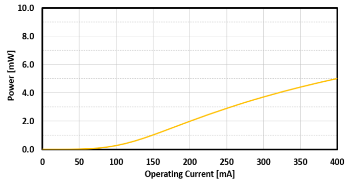
FIG. 6: SLED 2 OUTPUT POWER VS CURRENT
