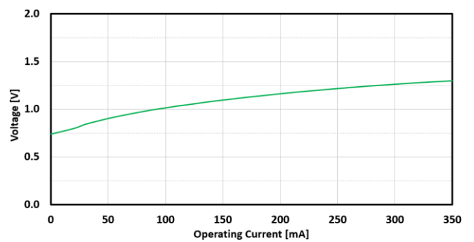
FIG. 8: SLED 1 FORWARD VOLTAGE VS CURRENT
