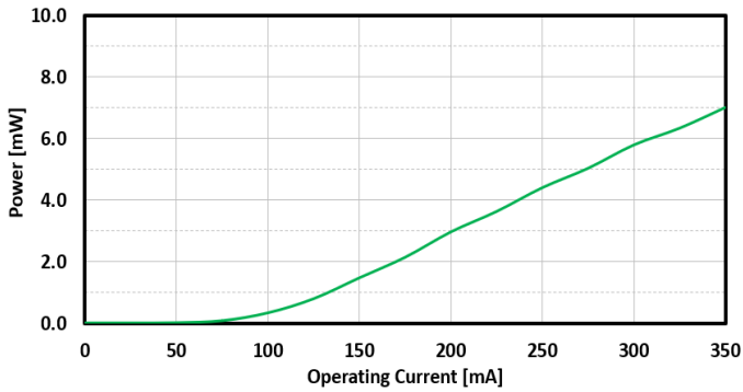
FIG. 5: SLED 1 OUTPUT POWER VS CURRENT
