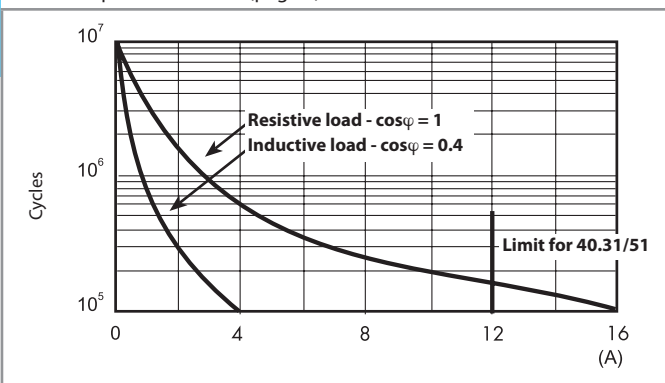
F 40.3 - Electrical life (AC) v contact current
