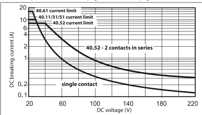
H 40.2 - Maximum DC1 breaking capacity
