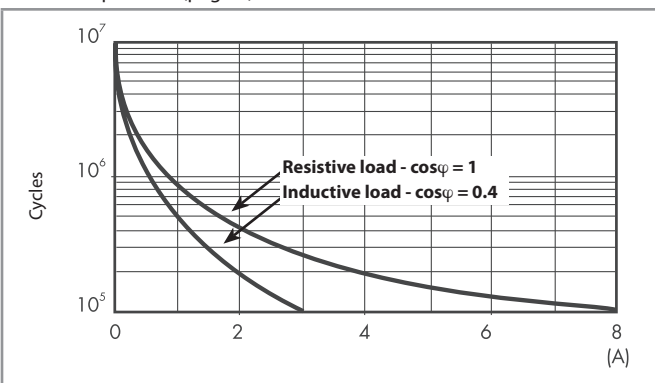
F 40.4 - Electrical life (AC) v contact current
