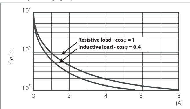
F 40.4 - Electrical life (AC) v contact current
