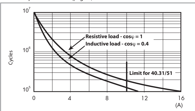
F 40.5 - Electrical life (AC) v contact current
