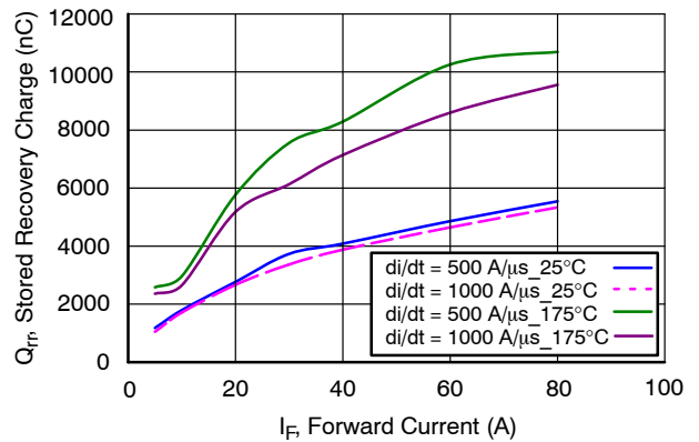
Figure 18. Stored Charge
