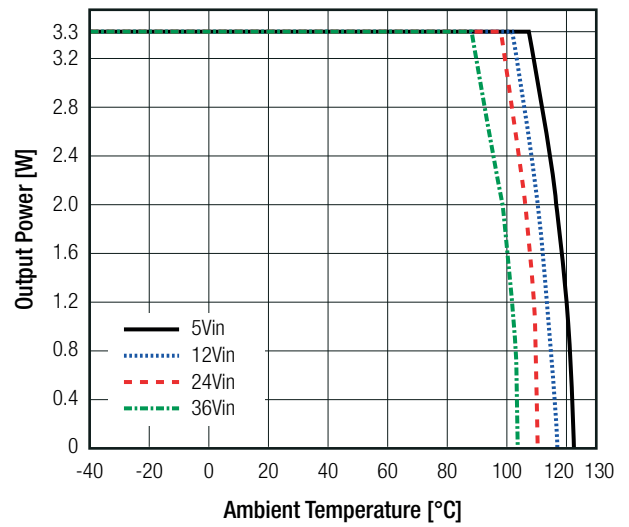
Thermal Derating
