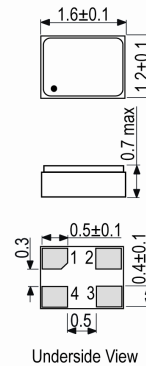
Underside View
