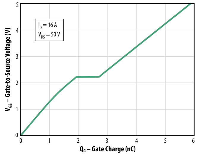
Figure 7: Gate Charge
