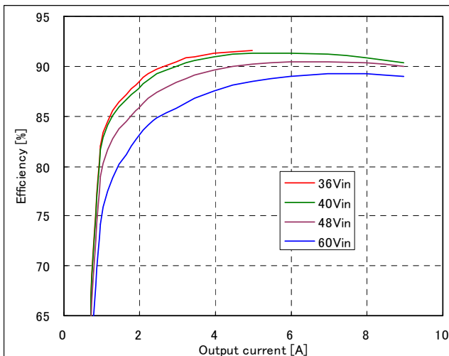
Fig.12V-2: Efficiency vs. load current and input voltage for converter mounted horizontally with airflow from pin 3 to pin 1 at a rate of 300LFM (1.5m/s) and Ta=25°C.
