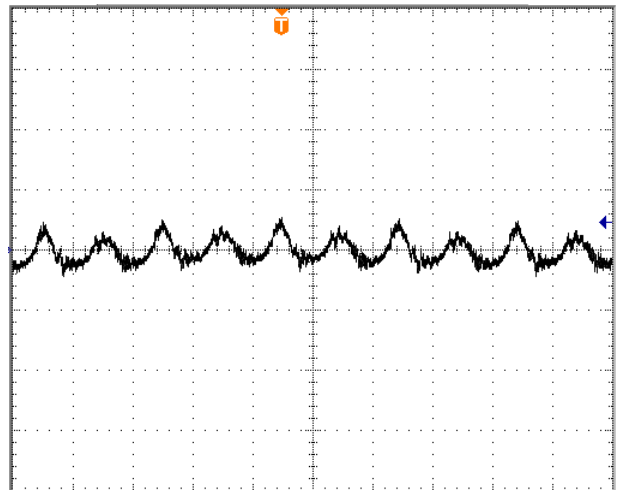
Fig.12V-7: Output voltage ripple (50mV/div) at full rated load current into a resistive load with Co=10uF tantalum + 1uF ceramic and Vin=48V. Time scale: 1us/div
