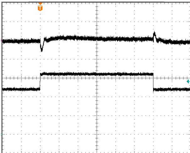
Fig.12V-6: Output voltage response to load current step-change (6.75A↔9A) at Vin=48V. Top trace: Output voltage (200mV/div). Bottom trace: load current (2.5A/div). Current slew rate: 5A/us. Co=100uF os-con + 10uF tantalum + 1uF ceramic. Time scale: 100us/div
