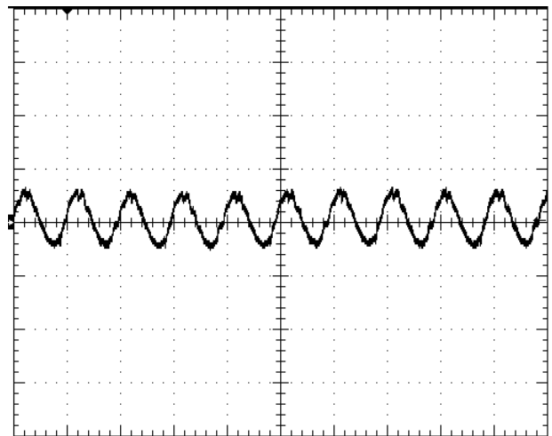
Fig.12V-10: Input reflected ripple current, I_c (200mA/div), measured through 10uH at the source at full rated load current and V_{in}=48V . Time scale: 1us/div.
