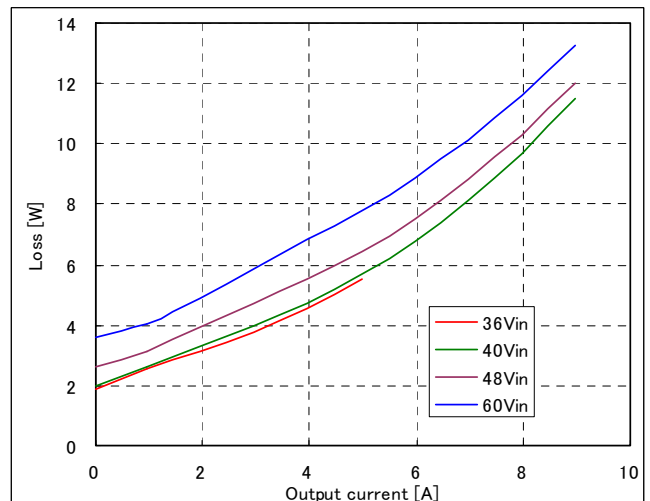
Fig.12V-3: Power Loss vs. load current and input voltage for converter mounted horizontally with airflow from pin 3 to pin 1 at a rate of 300LFM (1.5m/s) and Ta=25°C.
