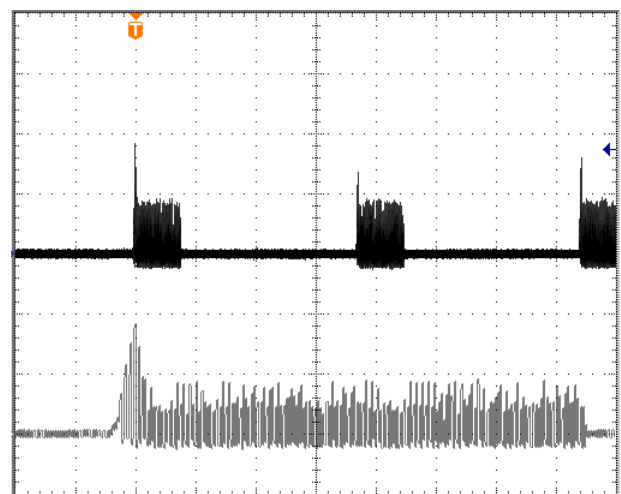
Fig.12V-12: Load current (top trace, 20A/div, 40ms/div) into a 10mΩ short circuit during restart, at V_{in} = 48V . Bottom trace (20A/div, 4ms/div) is an expansion of the top trace.
