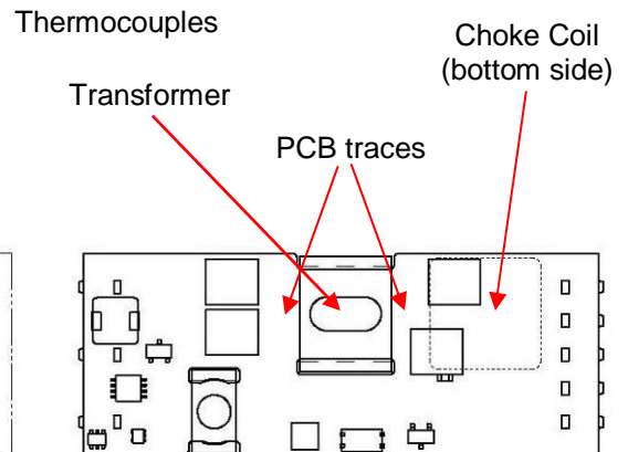
Fig. G: Location of thermocouples for thermal testing
