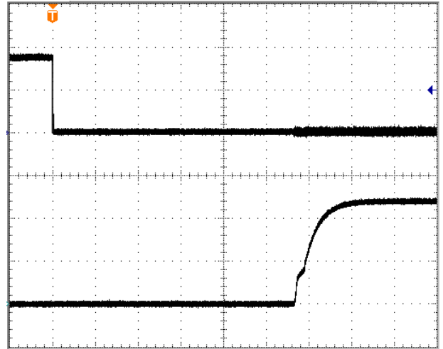
Fig.12V-5: Turn-on transient at full rated load current (resistive) plus 5,000uF at Vin=48V, triggered via ON/OFF pin. Top trace: ON/OFF signal (2V/div). Bottom trace: output voltage (5V/div). Time scale: 20ms/div
