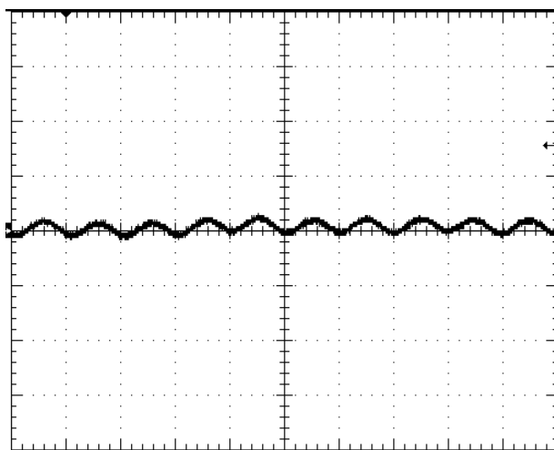
Fig.12V-9: Input reflected ripple current, I_s (10mA/div), measured through 10uH at the source at full rated load current and V_{in}=48V . Time scale: 1us/div.
