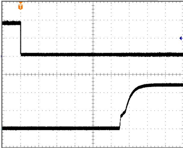
Fig.12V-4: Turn-on transient at full rated load current (resistive) with 10uF tantalum + 1uF ceramic capacitor at Vin=48V, triggered via ON/OFF pin. Top trace: ON/OFF signal (2V/div). Bottom trace: output voltage (5V/div). Time scale: 20ms/div
