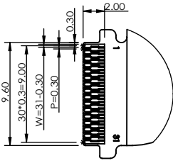
DETAILED VIEW A SCALE 2 : 1
