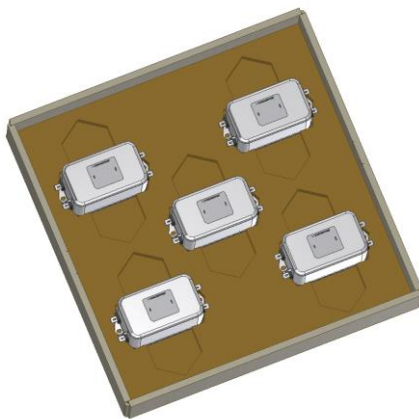
Figure 1: Example of old tray
