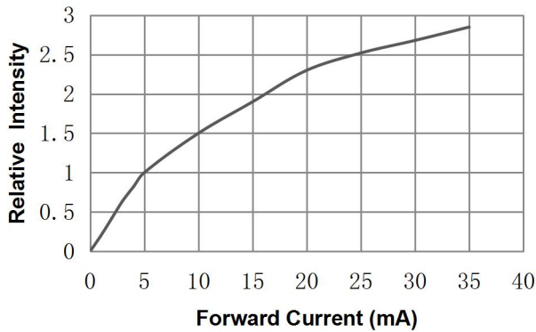
Relative Intensity VS. Forward Current ( T_a=25^\circ\text{C} )
