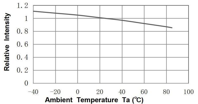
Relative Intensity VS. Ambient Temperature ( T_a=25^\circ\text{C} )
