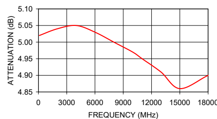
BW-S5W5+ ATTENUATION
