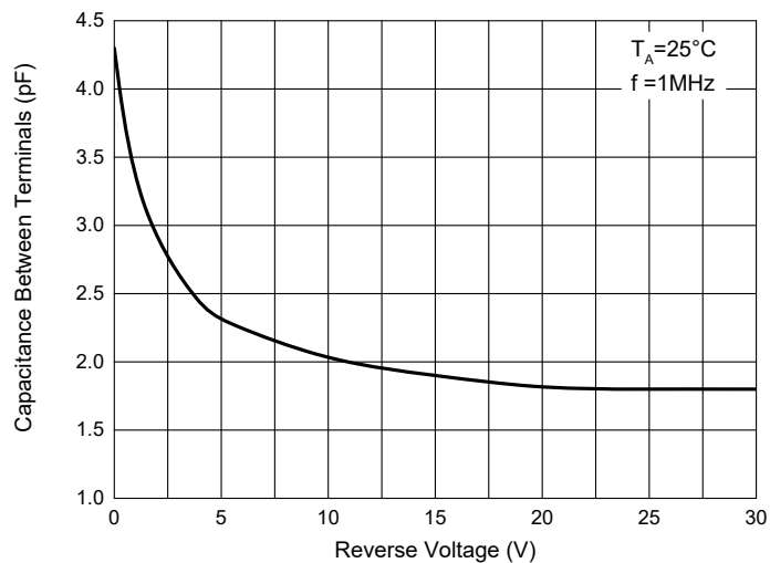
Fig. 3 - Capacitance Characteristics
