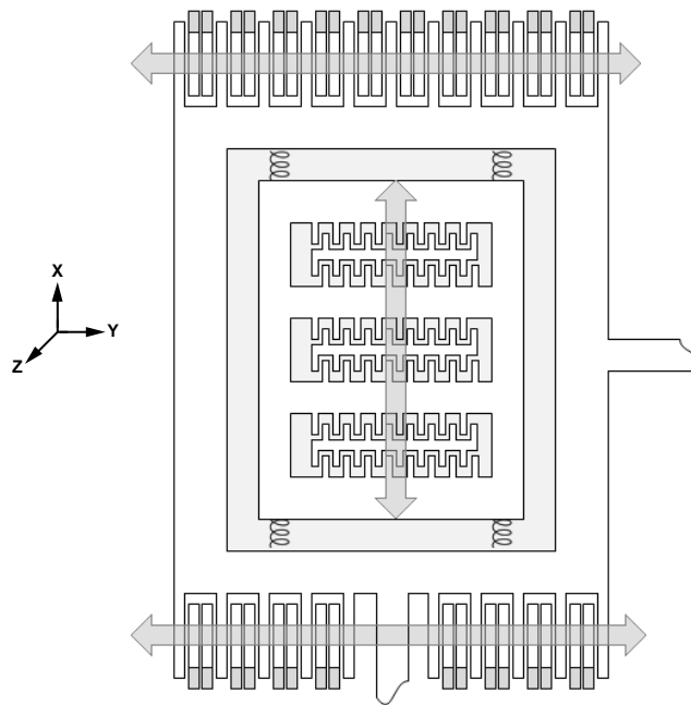
Figure 18. Simplified Gyro Sensing Structure—One Corner
