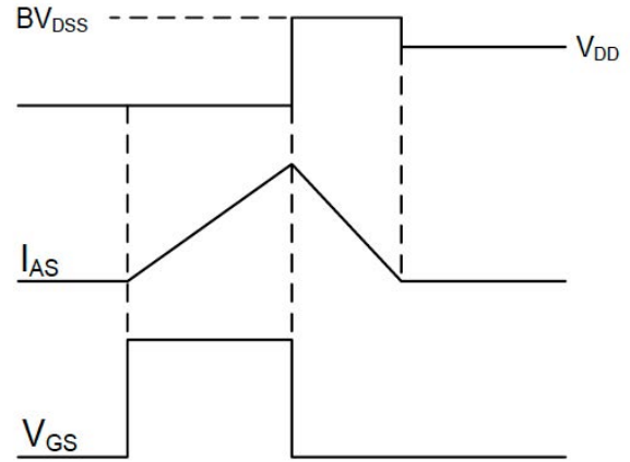
Figure 8. EAS Waveform
