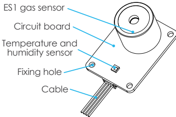
PS4 gas sensor
