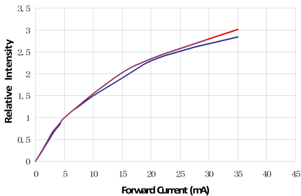
Relative Intensity VS. Forward Current ( T_a=25^\circ\text{C} )
