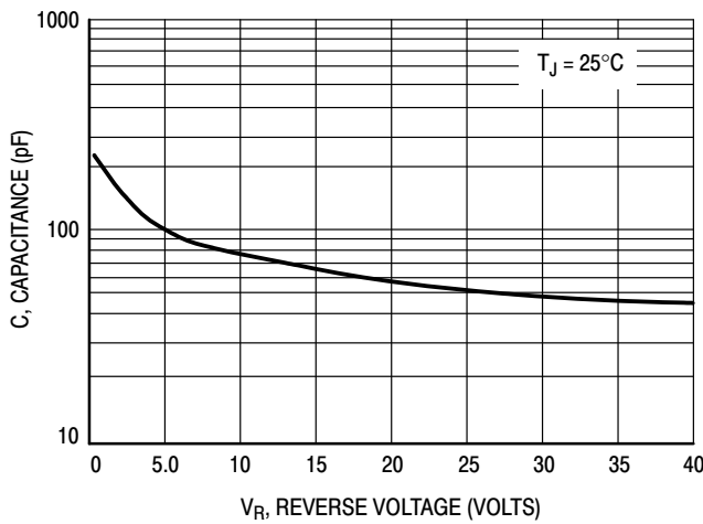
Figure 5. Capacitance
