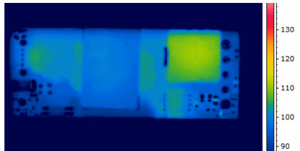
Figure 6. Thermal Image of CPE5C36 (5A output, 70C Ambient, 200lfm airflow, Vin = 48V, airflow from pin 3 to pin 1, Tmax = 109°C)
