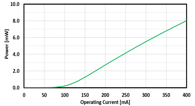
FIG. 6: SLED 1 OUTPUT POWER VS CURRENT
