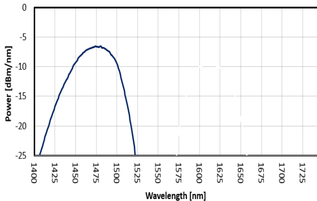
FIG. 5: SLED 4 SPECTRUM
