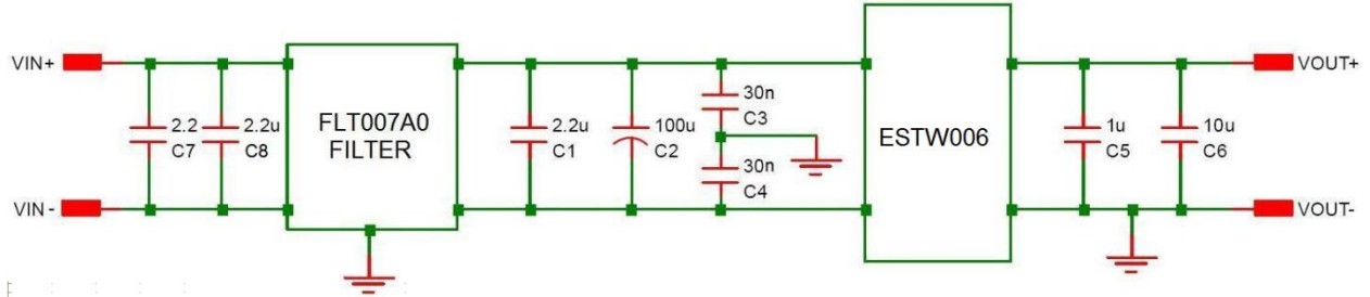
Figure 25. EMC Considerations.
