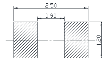
推荐焊盘尺寸 Recommended Soldering Pad
