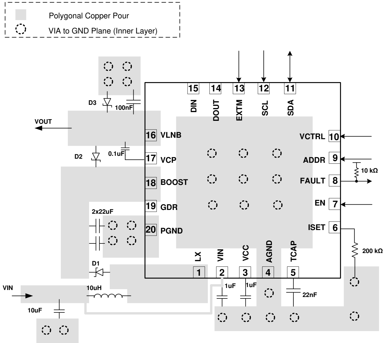
Figure 10-1. Layout
