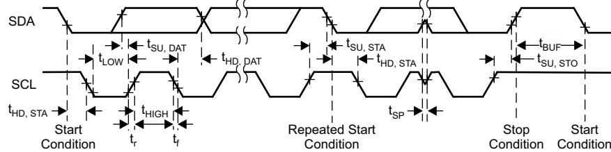
Figure 7-9. I 2 C Interface Timing Diagram
