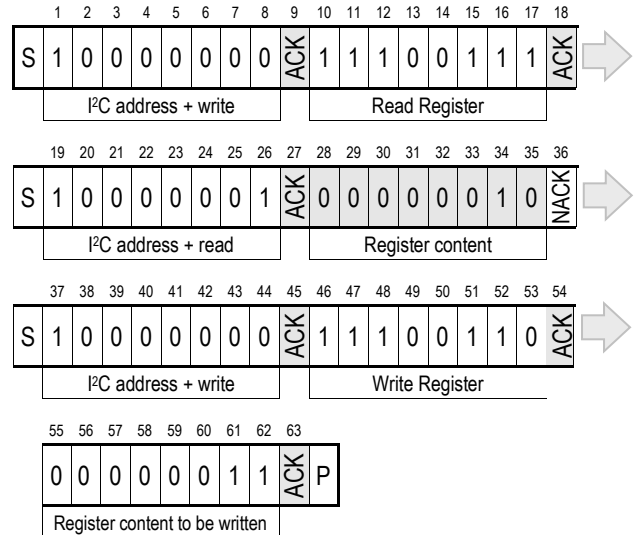
Figure 18 Read and write register sequence – grey blocks are controlled by SHT2x. In this example, the resolution is set to 8bit / 12 bit.
