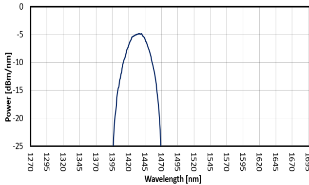
FIG. 5: SLED 4 SPECTRUM
