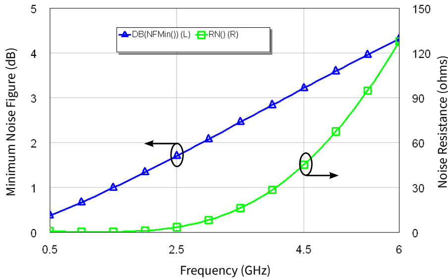
Figure 5. Simulated Minimum Noise Figure and Noise Resistance vs Frequency of the CGH40120P V_{DD} = 28\text{ V}, I_{DQ} = 1\text{ A}
