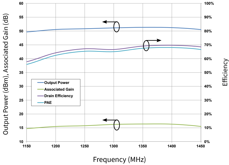
Figure 3. Associated Gain, Output Power, Drain Efficiency and PAE vs Frequency measured in Broadband Amplifier Circuit CGH40120P-AMP V_{DD} = 28\text{ V} , I_{DQ} = 1.0\text{ A}
