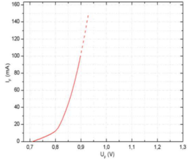
Forward current vs. forward voltage (typical)
