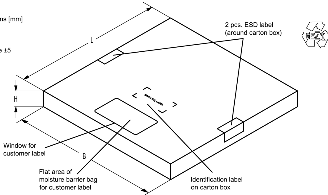
Figure 8: Drawing of folding box for reel with diameter of 180 mm.
