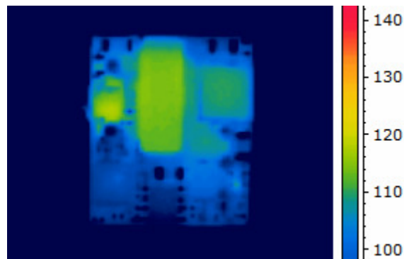
Figure 6. Thermal Image of CPZ4A36 4A output, 70C Ambient, 200lfm airflow, Vin = 48V, T max = 118°C
