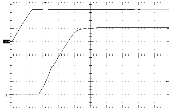
Figure 10. Startup Waveform via Input Voltage, time scale 4mS/div. Vin=Vin_nom, Iout=no load Cout=2000uF, Ch1=Vout (1V/div), Ch2=Vin (20V/div)
