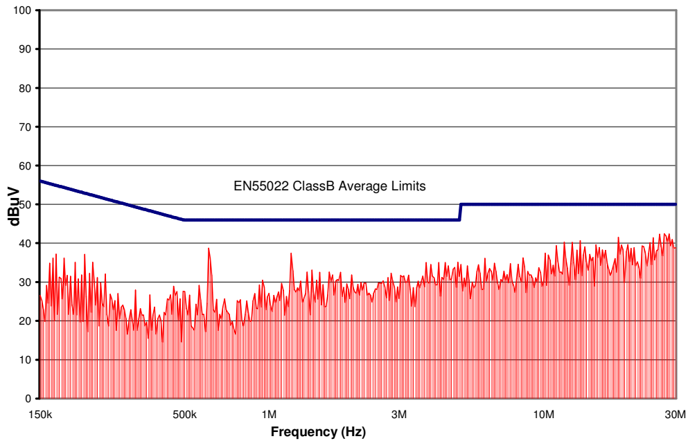
Figure 23. CPZ4A36 Conducted Emissions using above specified input filter, Vin = 48V, Full Resistive Load
