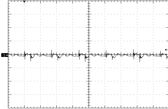
Figure 7. Output Voltage Ripple (20mV/div), time scale - 1uS/div. Vin=Vin_nom, full load Cout=1uF ceramic + 100uF Ceramic (see Fig 18)
