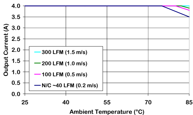
Figure 4. Output Current Derating vs Ambient Temperature & Airflow (converter mounted vertically with air flowing from pin 3 to pin 1, Vin = 24-36 V.)
