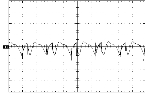
Figure 8. . Output Voltage Ripple (20mV/div), time scale - 1uS/div. Vin=Vin_nom, full load Cout=1uF ceramic + 10uF Tantalum (see Fig 19)
