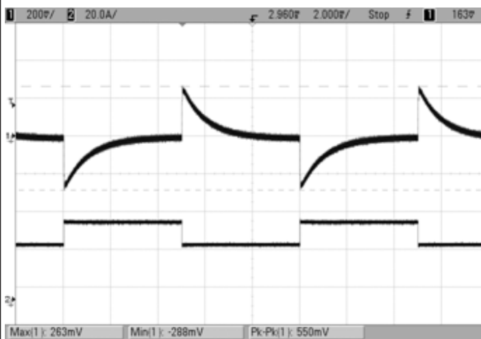
Step Load Transient Response (Vin=48V, Vout=nom, Cload= 1uF || 10uF, Iout=50 to 75 to 50% of full load, Ta=+25°C) Ch1=Vout, Ch2=Iout.
