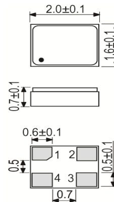
Underside View
