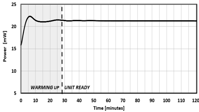
FIG. 9: WARM-UP TIME
