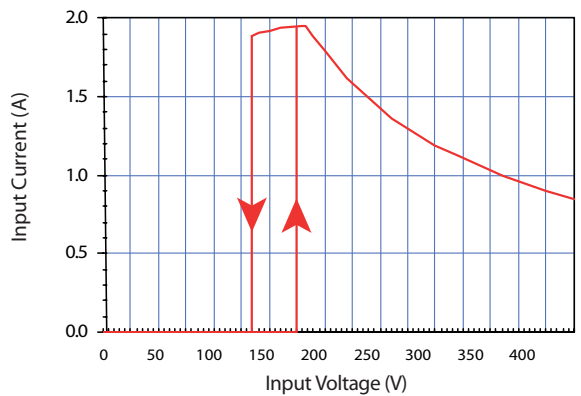
INPUT CHARACTERISTIC, I_{out} = 25A, T_c=25^\circ C
