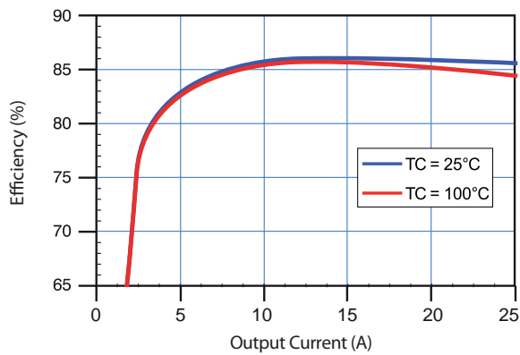
EFFICIENCY VS. LOAD, V_{in}=300V
