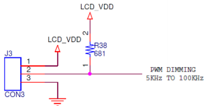
OPTIONAL PROCESSOR PWM BACKLIGHT CONTROL
