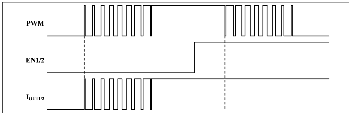
Figure 64 Priority Logic 2 of EN1/2 in Level Control Mode
