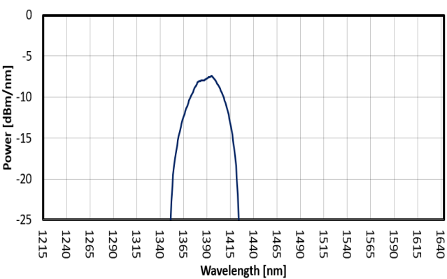
FIG. 5: SLED 4 SPECTRUM
