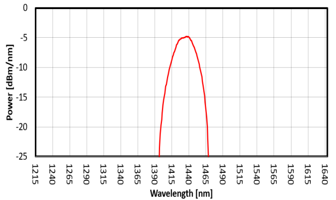
FIG. 6: SLED 5 SPECTRUM
