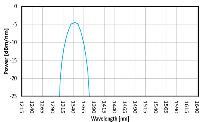
FIG. 6: SLED 5 SPECTRUM
