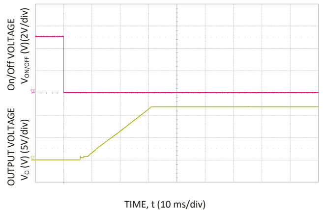
Figure 6. Typical Start-Up Using Remote On/Off with Vin applied, negative logic version shown.
