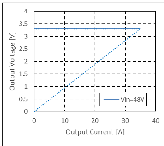
Fig-11: Output voltage vs. load current showing current limit point and power module shutdown point. ( V_{in} = 48V )
