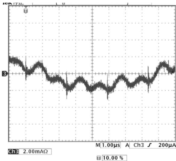
Fig-9: Input reflected ripple current, I_s (2mA/div), measured through 10uH at the source at full rated load current and V_{in}=48V . Time scale: 1us/div.
