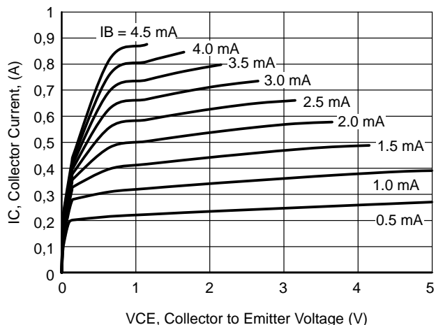
Figure 3. IC – VCE
