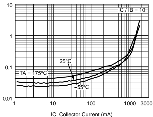
Figure 7. VCE(sat) – IC
