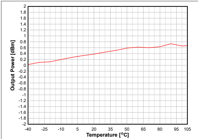
Figure 8-16. Output Power vs. Temperature (BLE 1 Mbps, 2.44 GHz, 0dBm)
