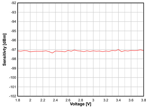
Figure 8-13. Sensitivity vs. Supply Voltage (VDD5) (BLE 1 Mbps, 2.44 GHz)
