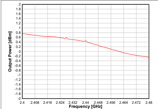
Figure 8-20. Output Power vs. Frequency (BLE 1 Mbps, 0dBm)
