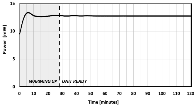
FIG. 7: WARM-UP TIME
