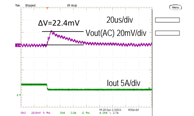
Step Load Transient Response (Vin=5.0V, Vout=1.8V, Cload=400uF, Iout=4A to 2A, 2.5A/us)
