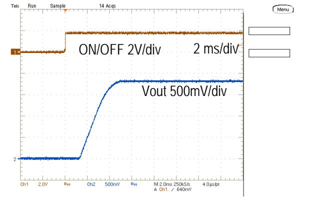
On/Off Enable Delay (Vin=5.0V, Vout=1.8V, Iout=4A, Cload=400uF)
