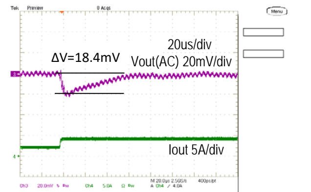
Step Load Transient Response (Vin=5.0V, Vout=1.8V, Cload=400uF, Iout=2A to 4A, 2.5A/us)
