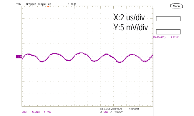
Output Ripple and Noise (Vin=5.0V, Vout=1.8V, Iout=4A, Cload=400uF, ScopeBW=20MHz)
