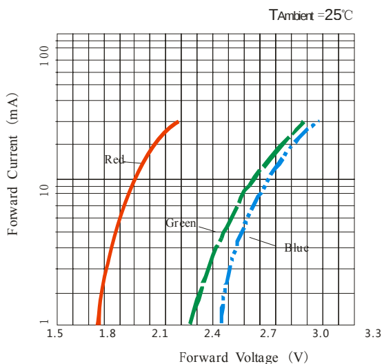
Volt-Ampere Characteristics
