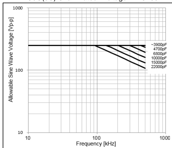
Chip(LxW): 3.2x1.6mm C0G(5C) Char. Rated Voltage : DC250V
