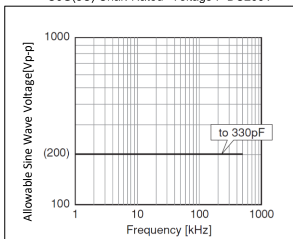
Chip(LxW): 2.0x1.25mm C0G(5C) Char. Rated Voltage : DC200V
