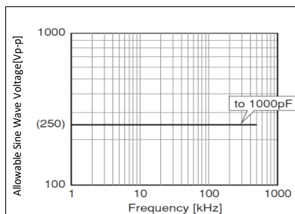
Chip(LxW): 1.6x0.8mm C0G(5C) Char. Rated Voltage : DC250V
