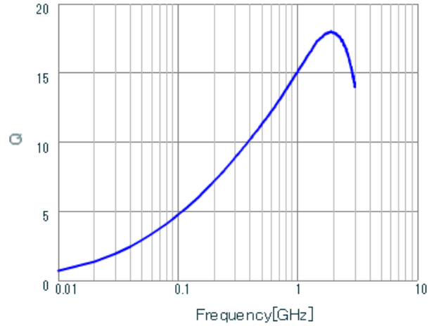
LQP02TN11NJ02 Q.
