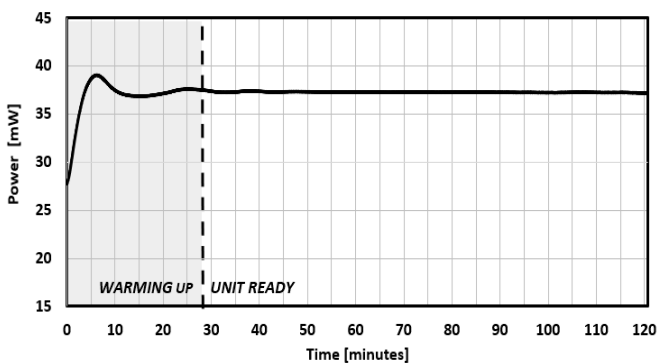
FIG. 13: WARM-UP TIME
