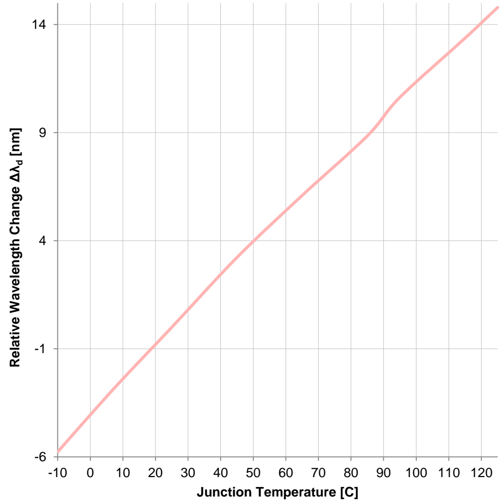
Junction Temperature vs. Peak Wavelength:
