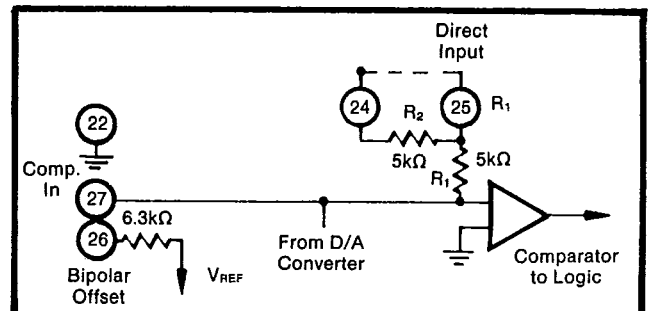
FIGURE 8. ADC76 Input Scaling Circuit.
