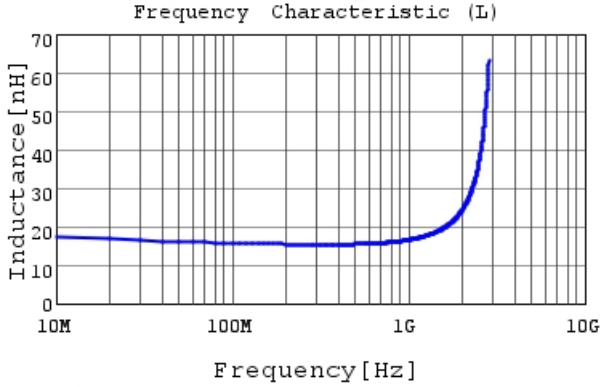
LQG15WZ16NG02 L
