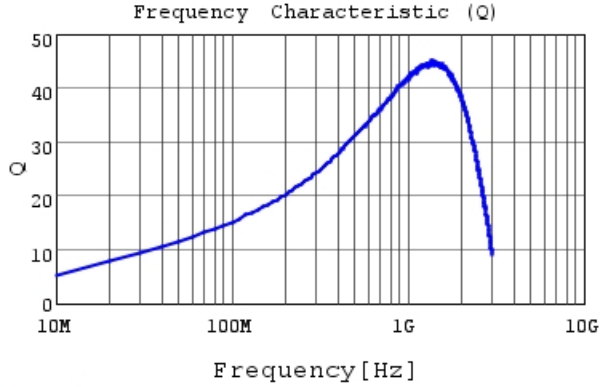
LQG15WZ16NG02 Q
