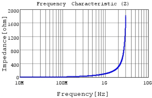
LQG15WZ16NG02 |Z|
