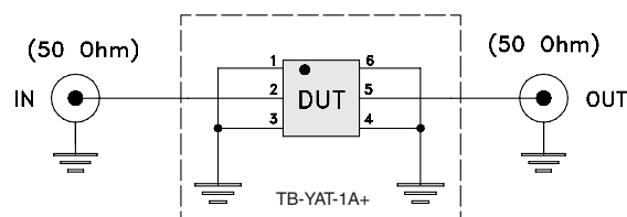
Fig 1. Block diagram of Test Circuit used for characterization, Test board TB-YAT-1A+ Conditions: Attenuation, VSWR: Pin=-10 dBm
