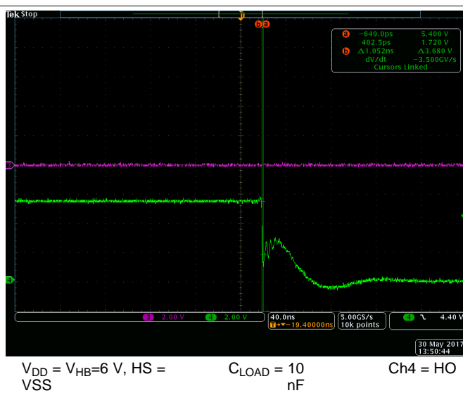
Figure 36. HO Fall Time
