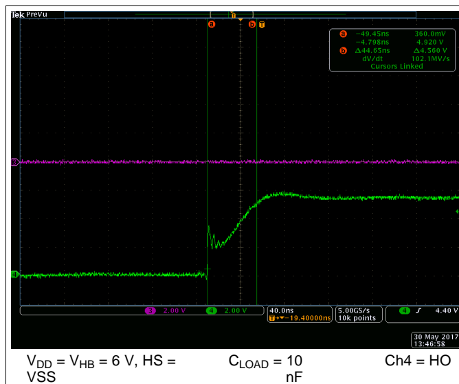
Figure 35. HO Rise Time
